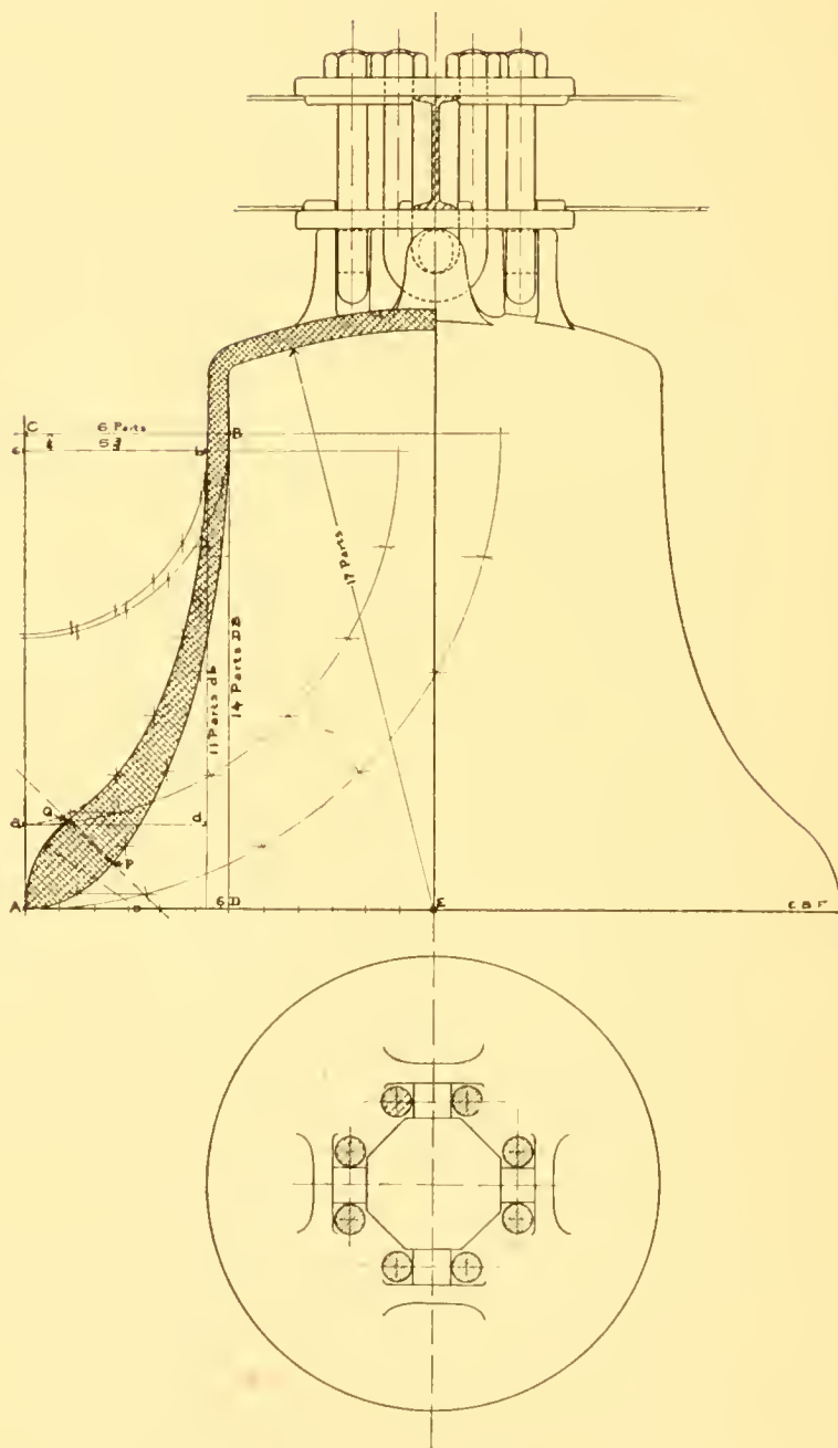
Fig. 15. Method of designing bells.
